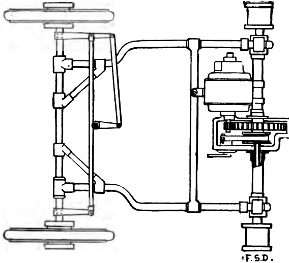
FIG. 68. —The Riker Underframe, showing the swivel connections at front and rear to permit distortion on uneven roads.
